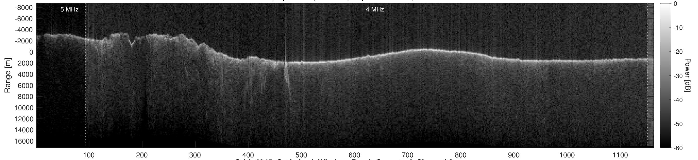
Orbit 4015, Optimized, Window, Depth-Corrected, Channel 2
