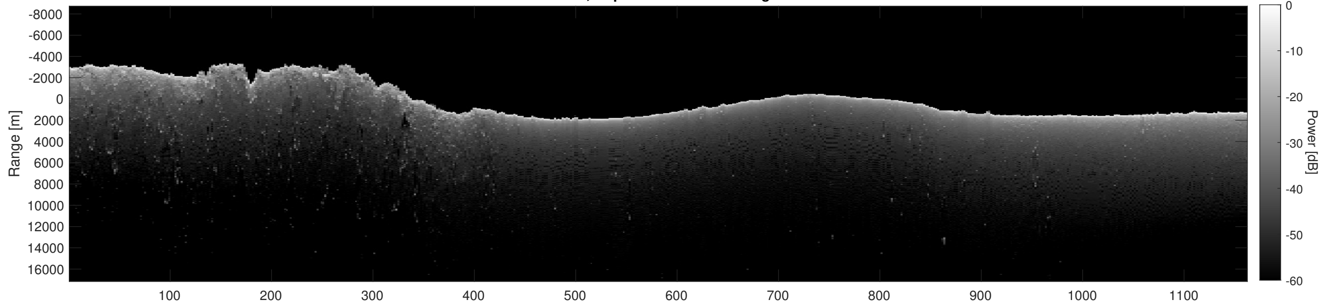
Orbit 4015, Depth-Corrected Cluttergram
