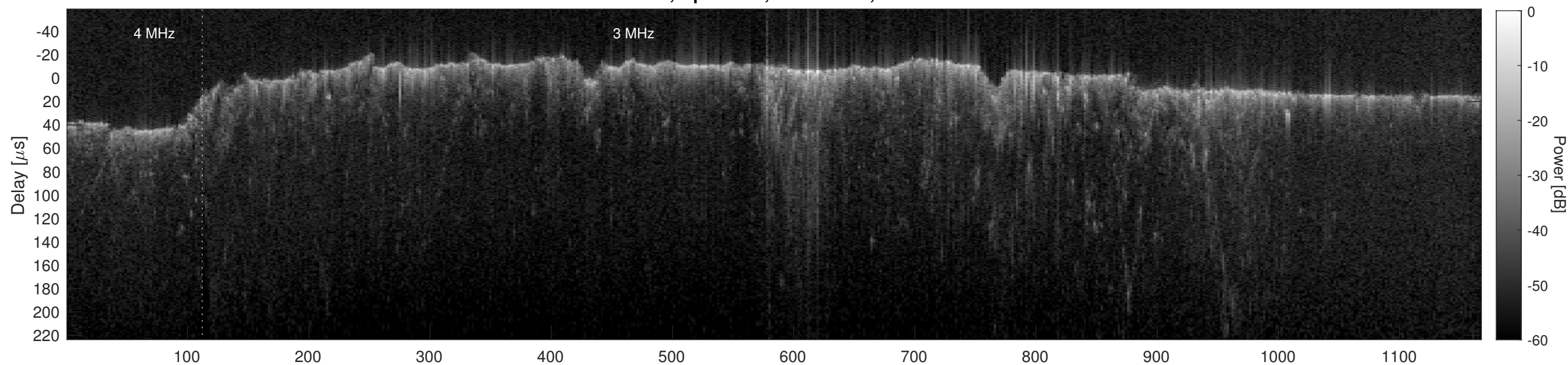
Orbit 4016, Cluttergram
