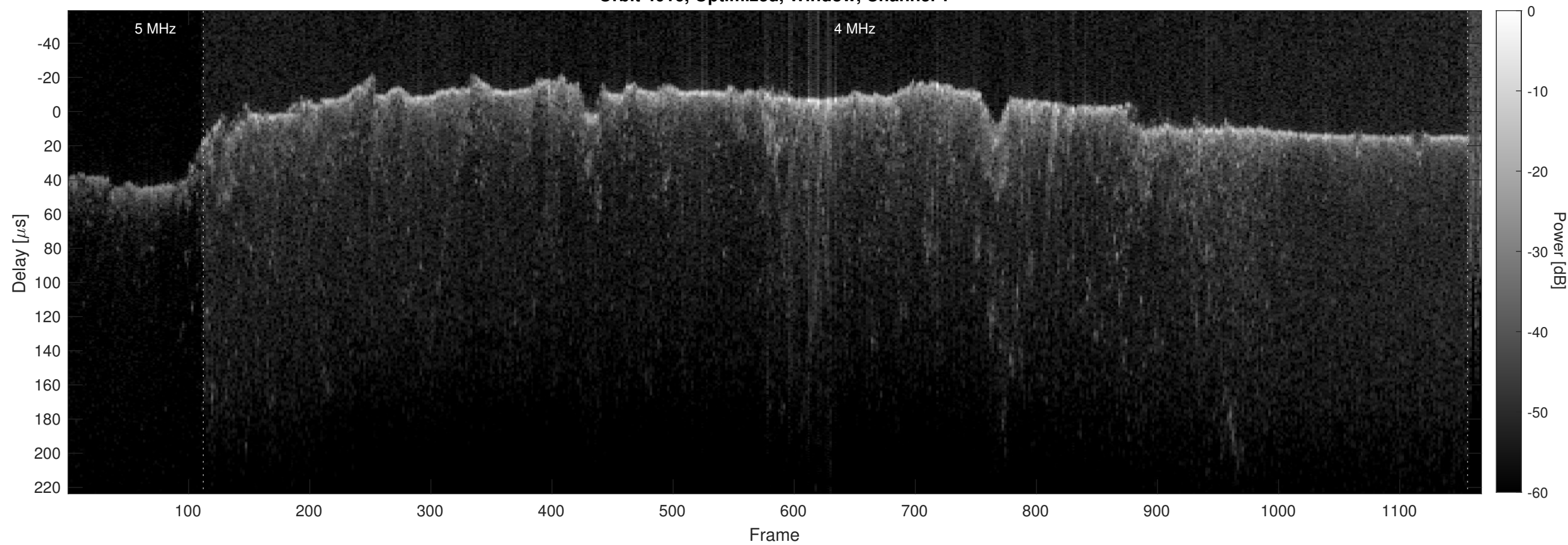
Orbit 4016, Optimized, Window, Channel 2
