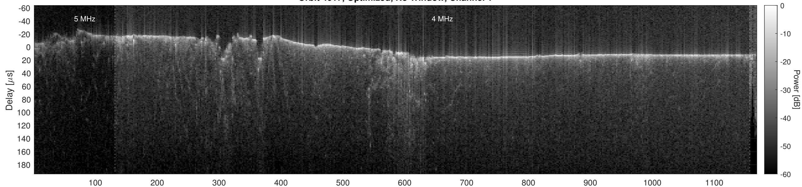
Orbit 4017, Optimized, No Window, Channel 2
