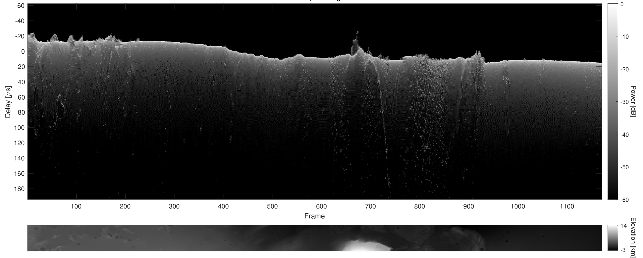
Orbit 4018, Cluttergram
