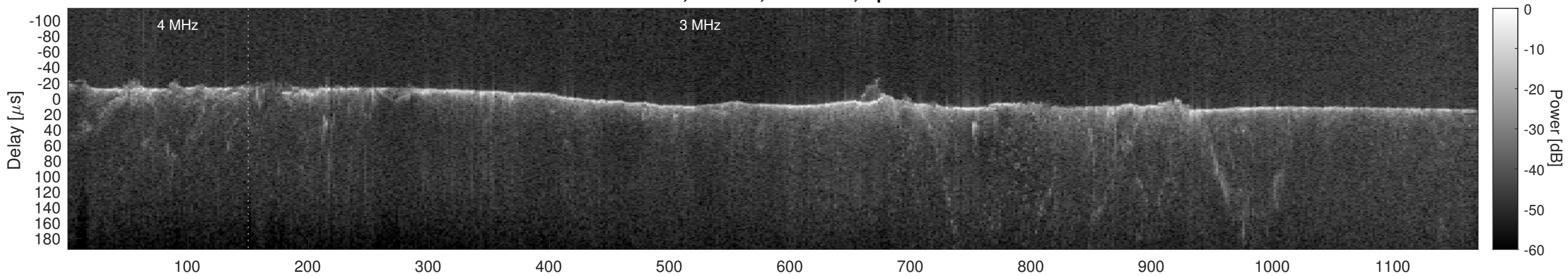
Orbit 4018, Cluttergram
