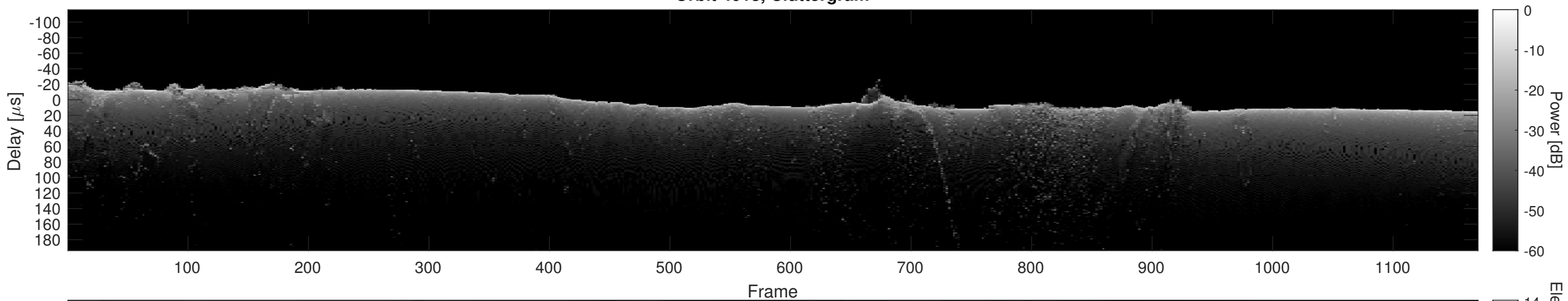
Orbit 4018, Cluttergram
