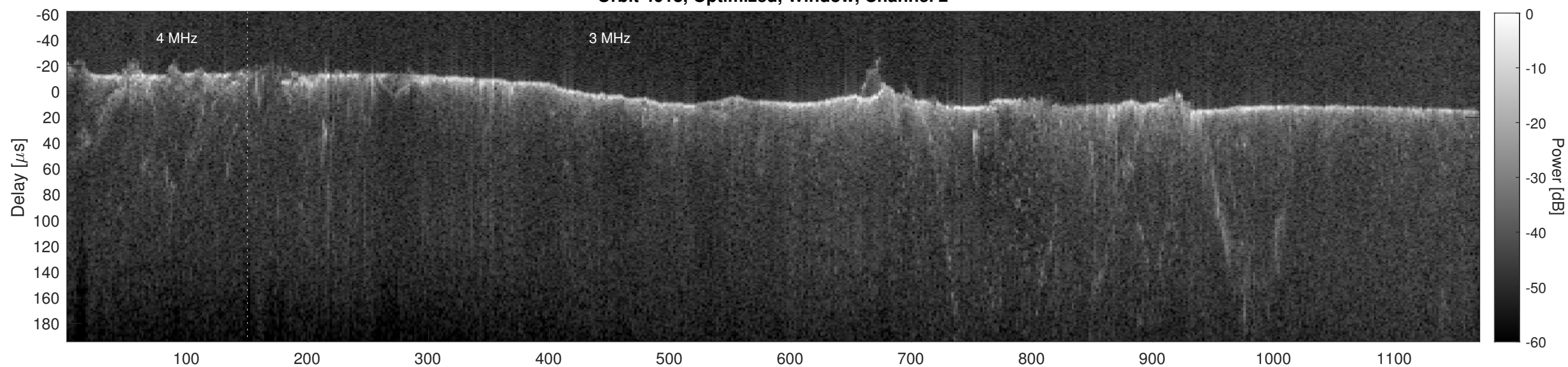
Orbit 4018, Cluttergram
