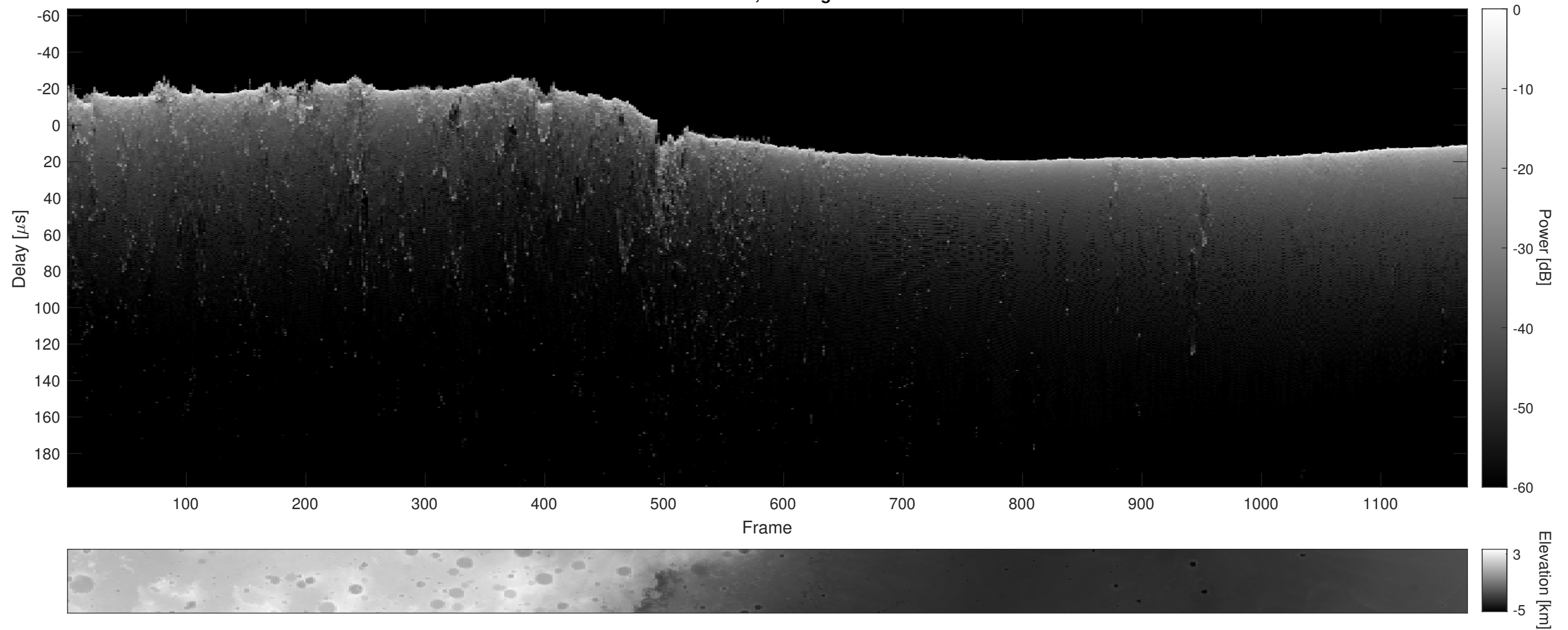
Orbit 4019, Cluttergram
