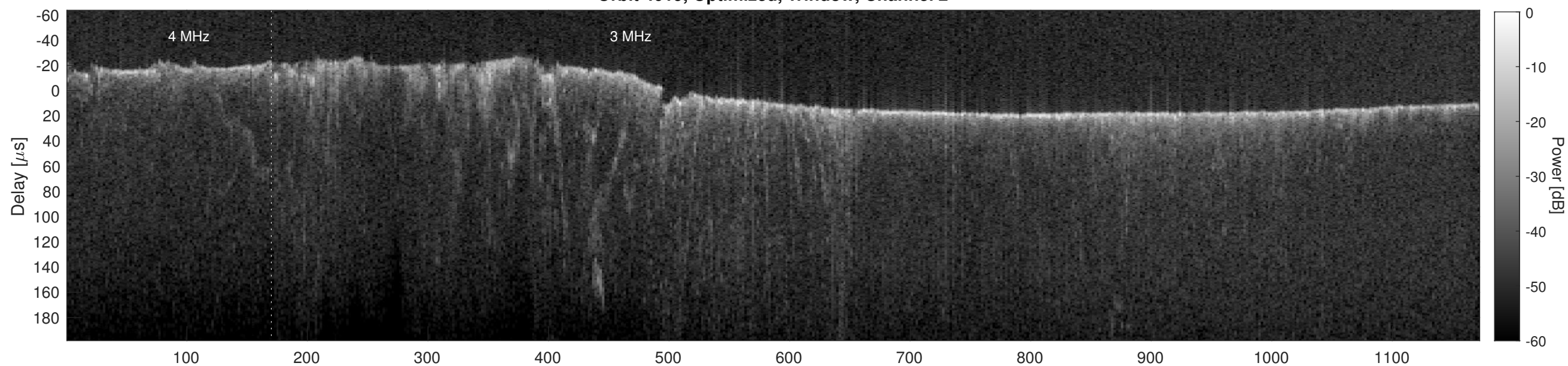
Orbit 4019, Cluttergram
