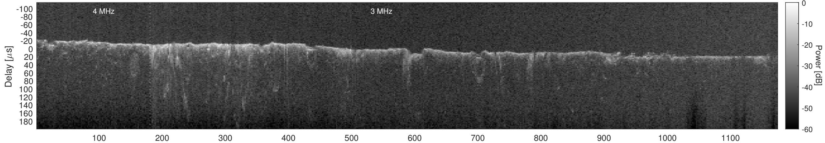
Orbit 4020, Cluttergram
