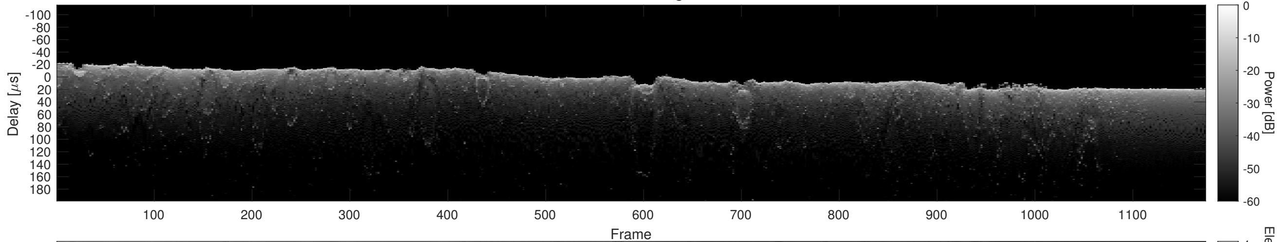
Orbit 4020, Cluttergram
