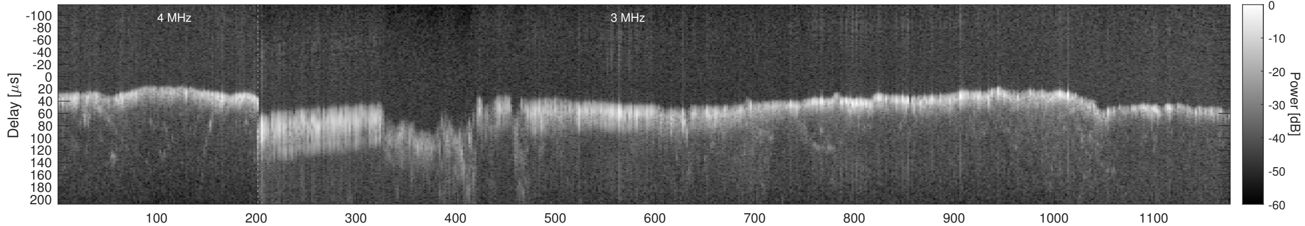
Orbit 4021, Window, Channel 2, Chapman
