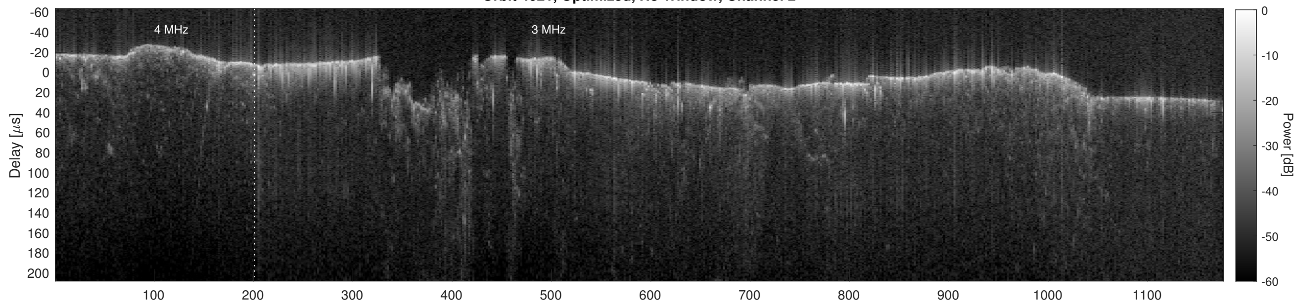
Orbit 4021, Cluttergram
