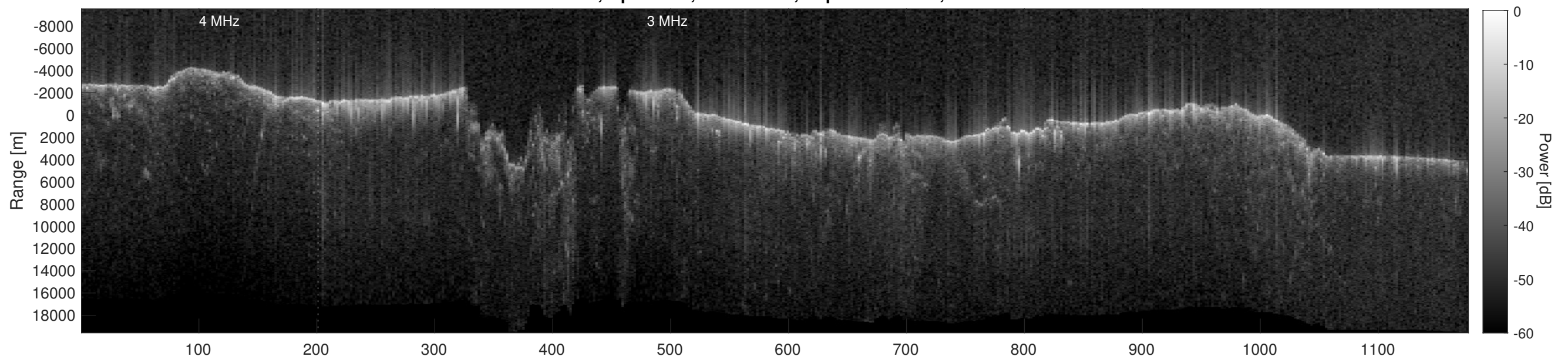
Orbit 4021, Depth-Corrected Cluttergram
