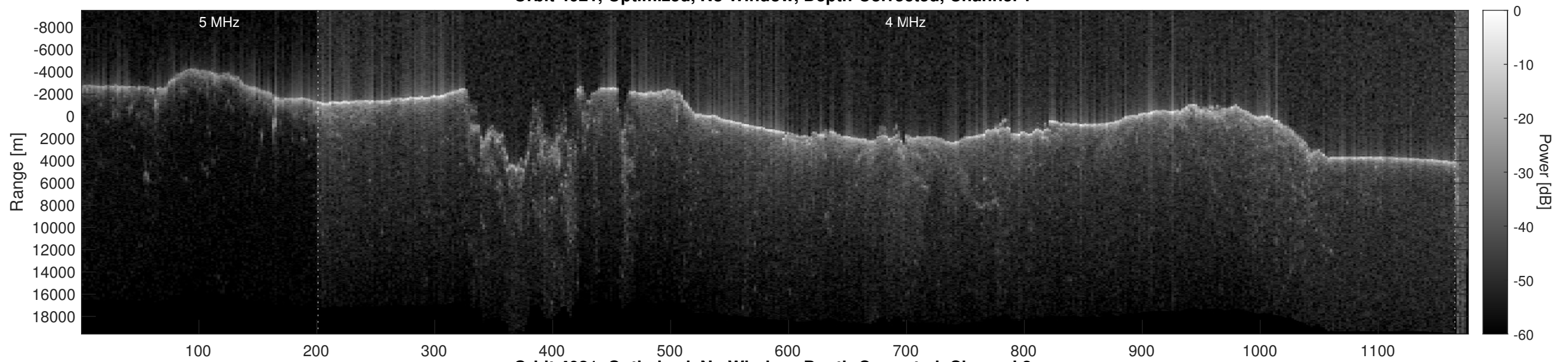
Orbit 4021, Optimized, No Window, Depth-Corrected, Channel 2
