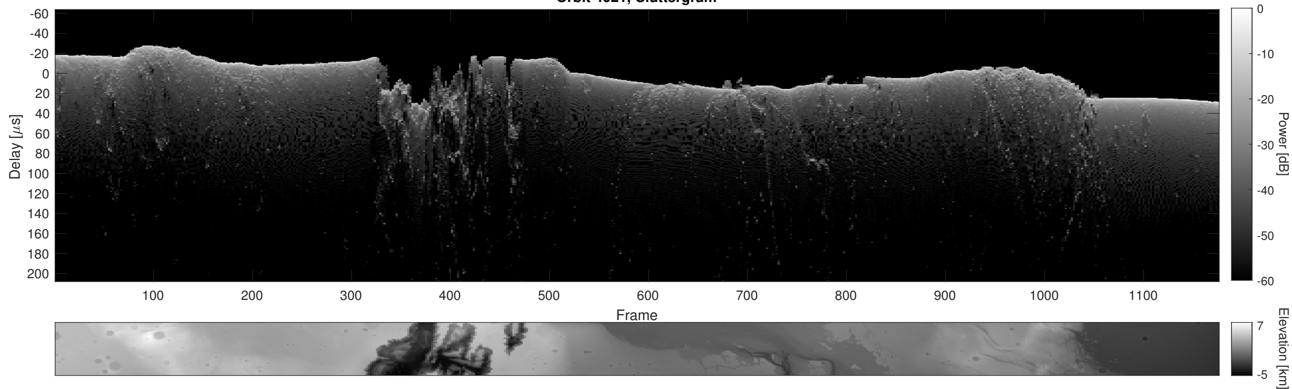
Orbit 4021, Cluttergram
