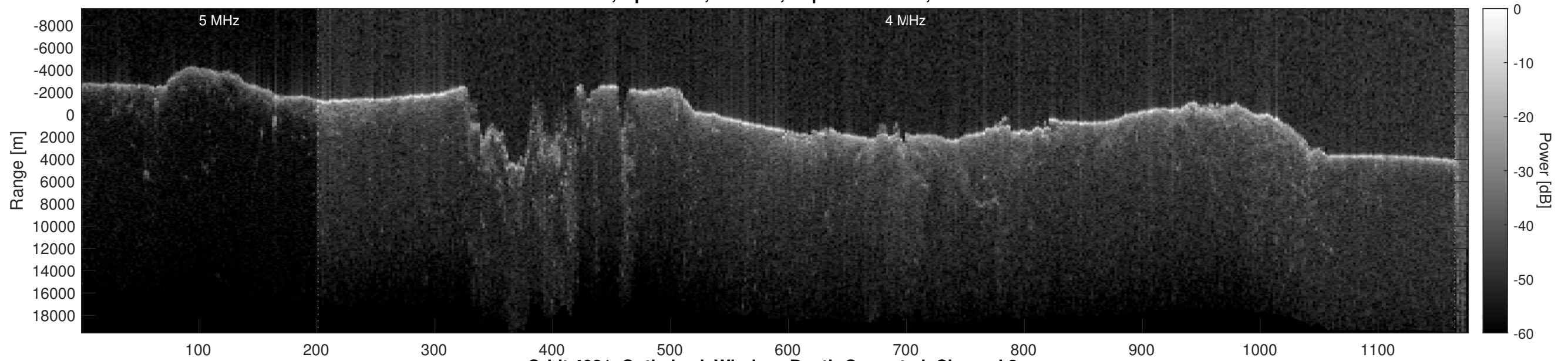
Orbit 4021, Optimized, Window, Depth-Corrected, Channel 2
