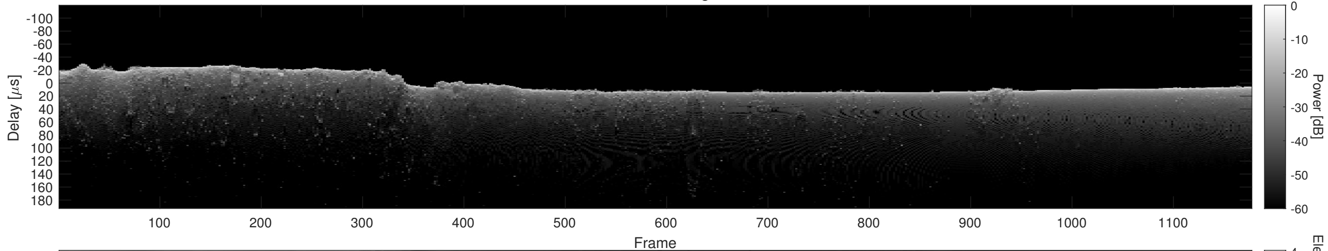
Orbit 4022, Cluttergram
