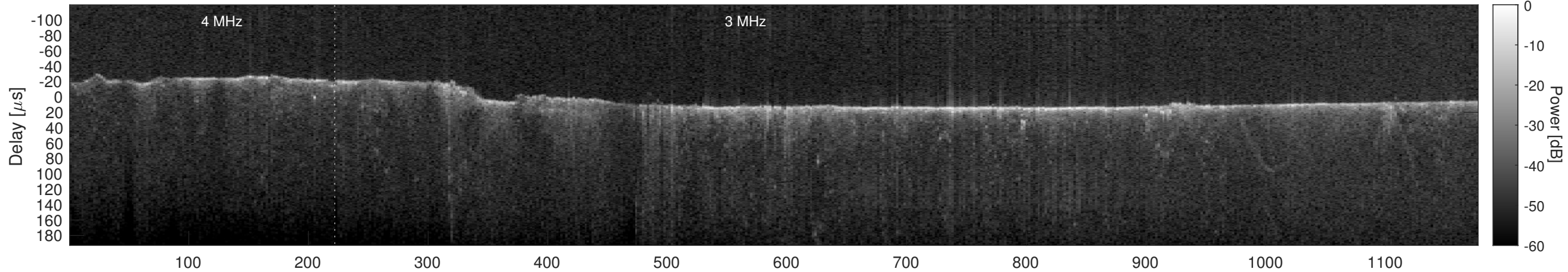
Orbit 4022, Cluttergram
