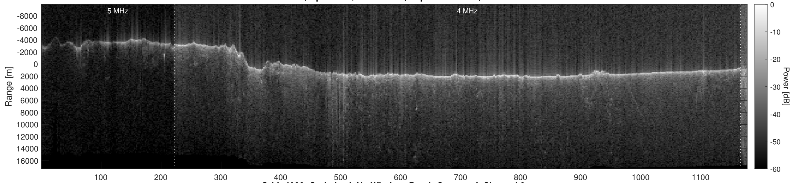
Orbit 4022, Optimized, No Window, Depth-Corrected, Channel 2
