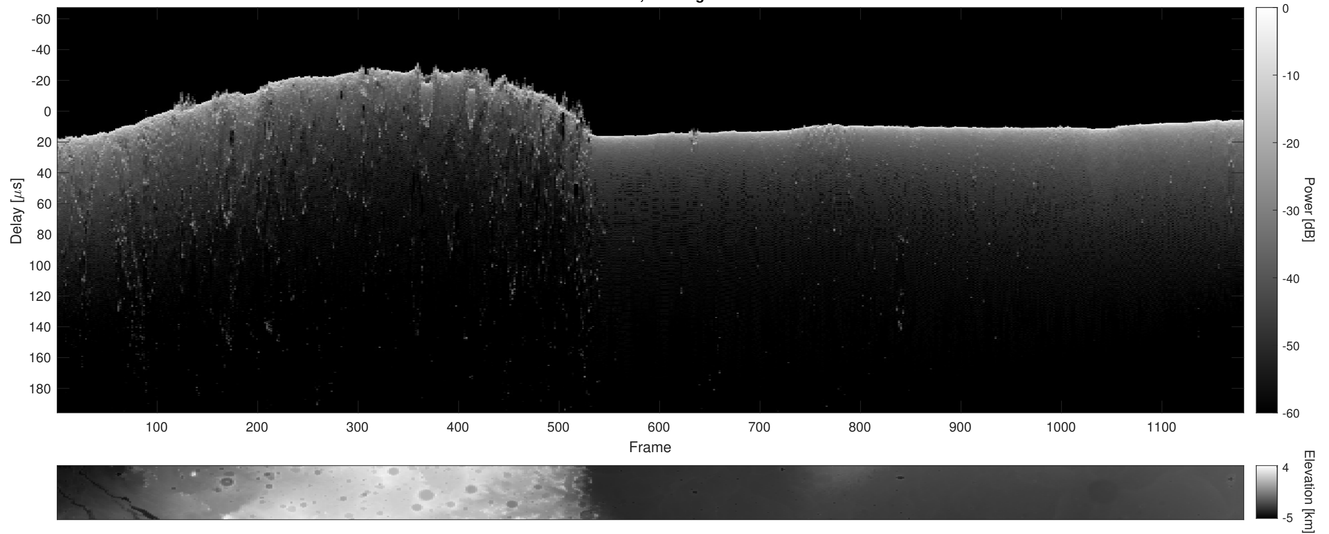
Orbit 4023, Cluttergram
