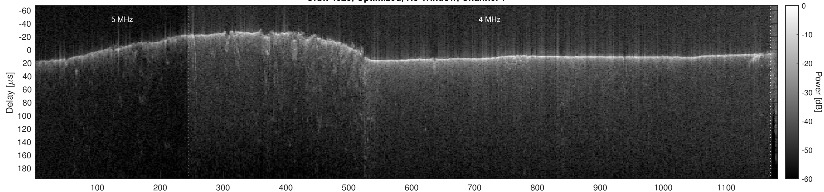
Orbit 4023, Optimized, No Window, Channel 2
