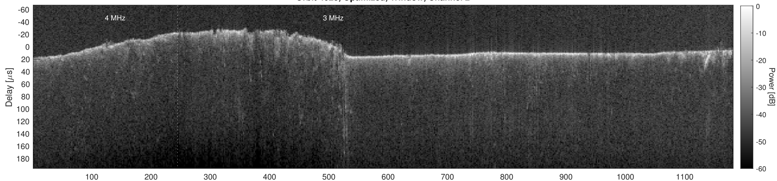
Orbit 4023, Cluttergram
