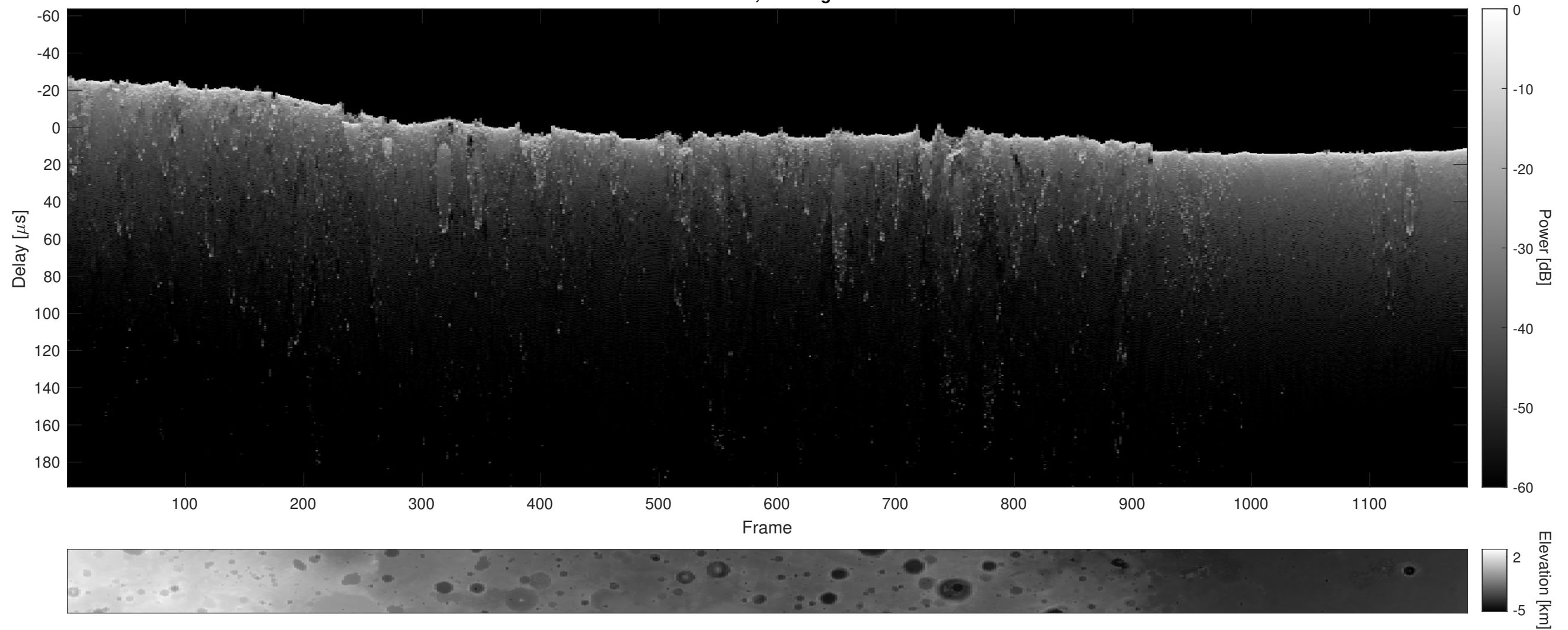
Orbit 4024, Cluttergram
