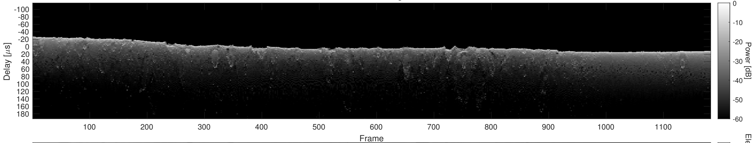
Orbit 4024, Cluttergram
