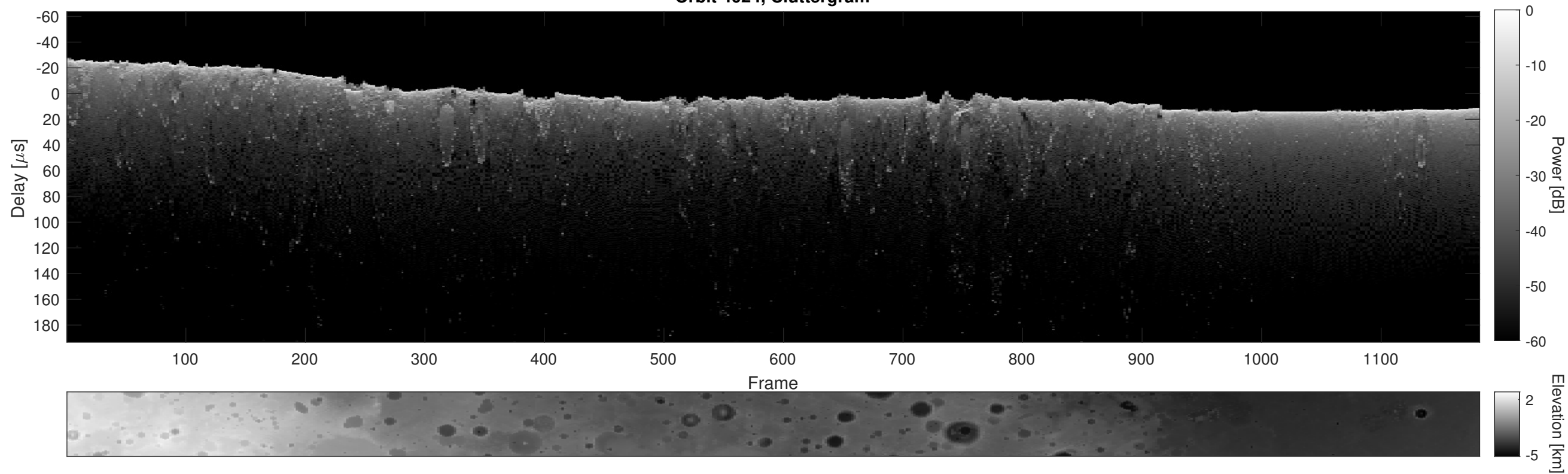
Orbit 4024, Cluttergram
