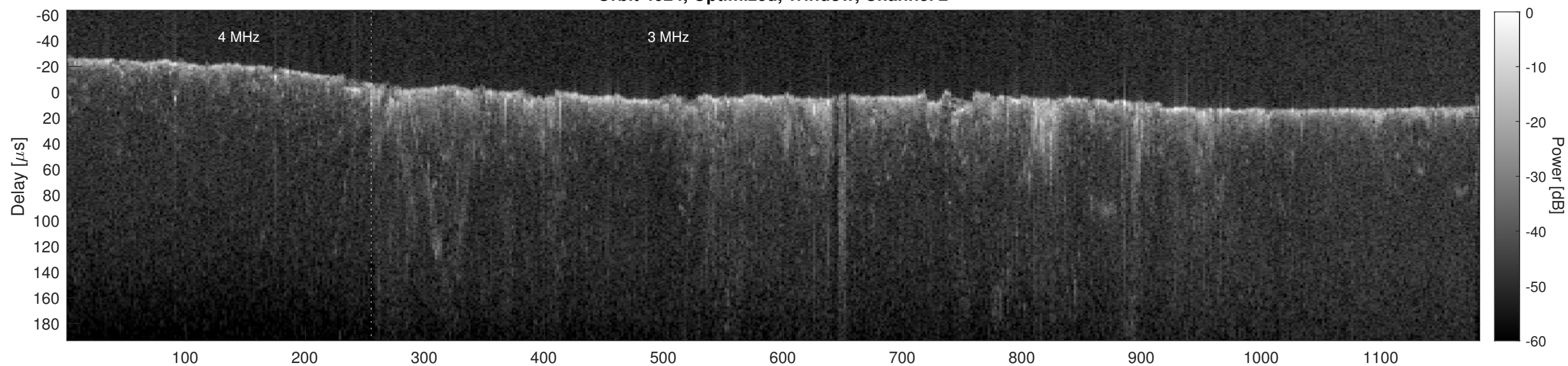
Orbit 4024, Cluttergram
