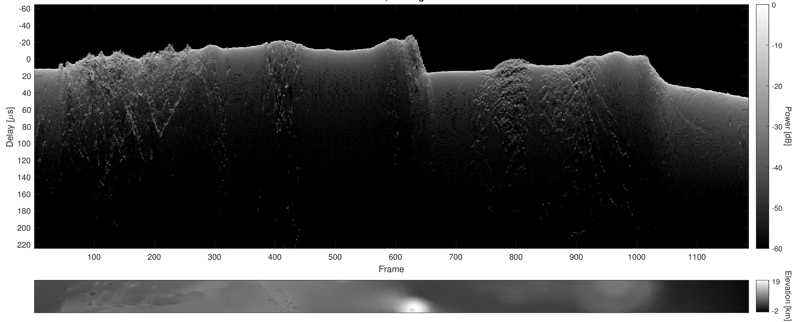
Orbit 4025, Cluttergram
