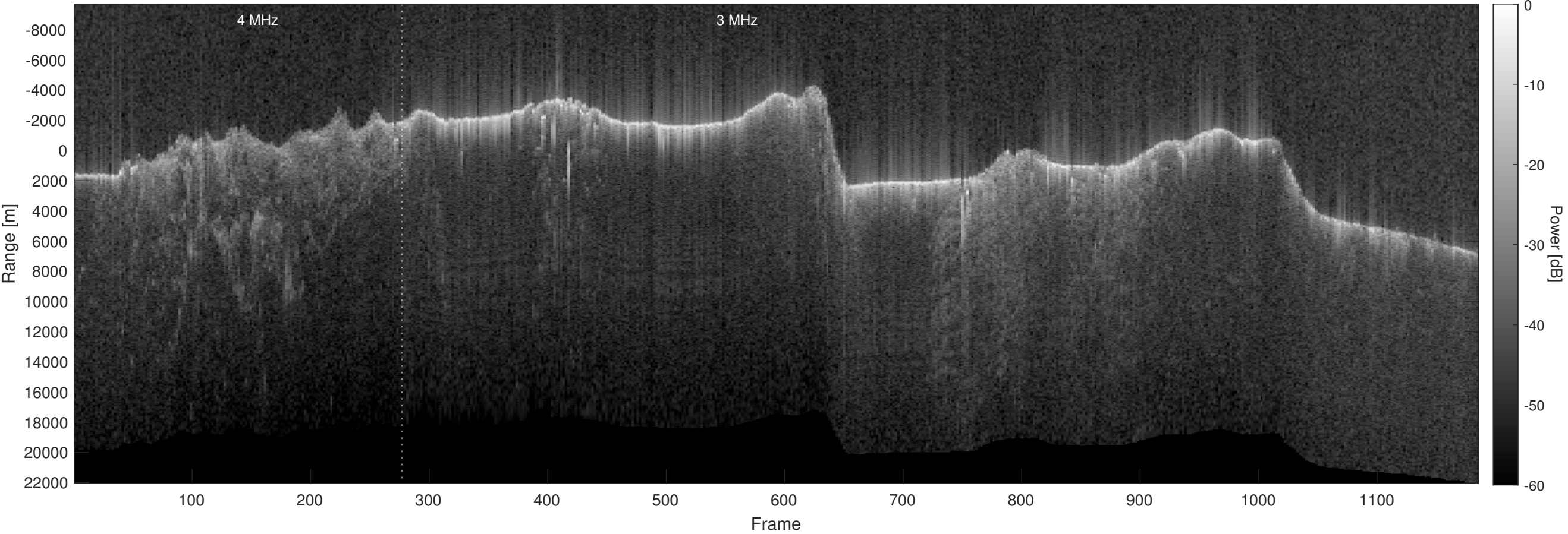
Orbit 4025, Optimized, No Window, Depth-Corrected, Channel 2
