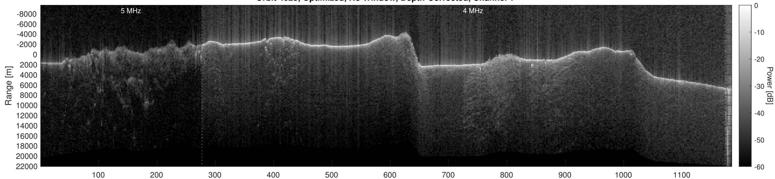
Orbit 4025, Optimized, No Window, Depth-Corrected, Channel 2
