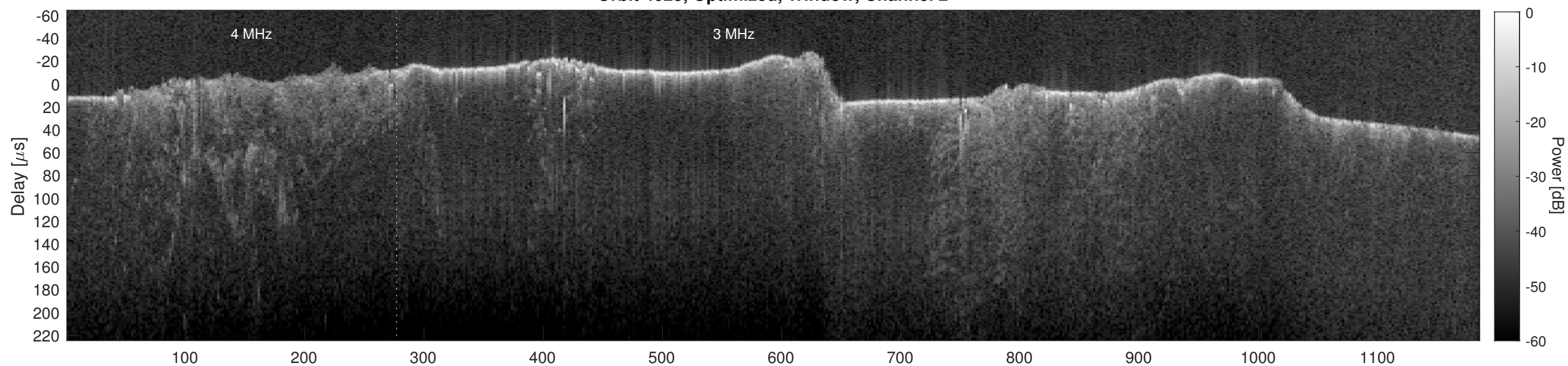
Orbit 4025, Cluttergram
