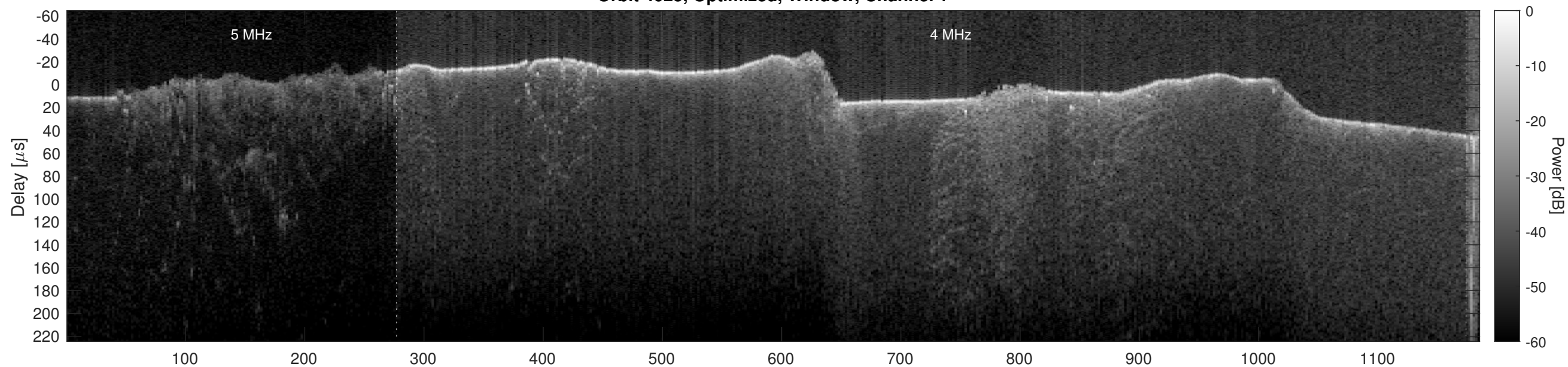
Orbit 4025, Optimized, Window, Channel 2
