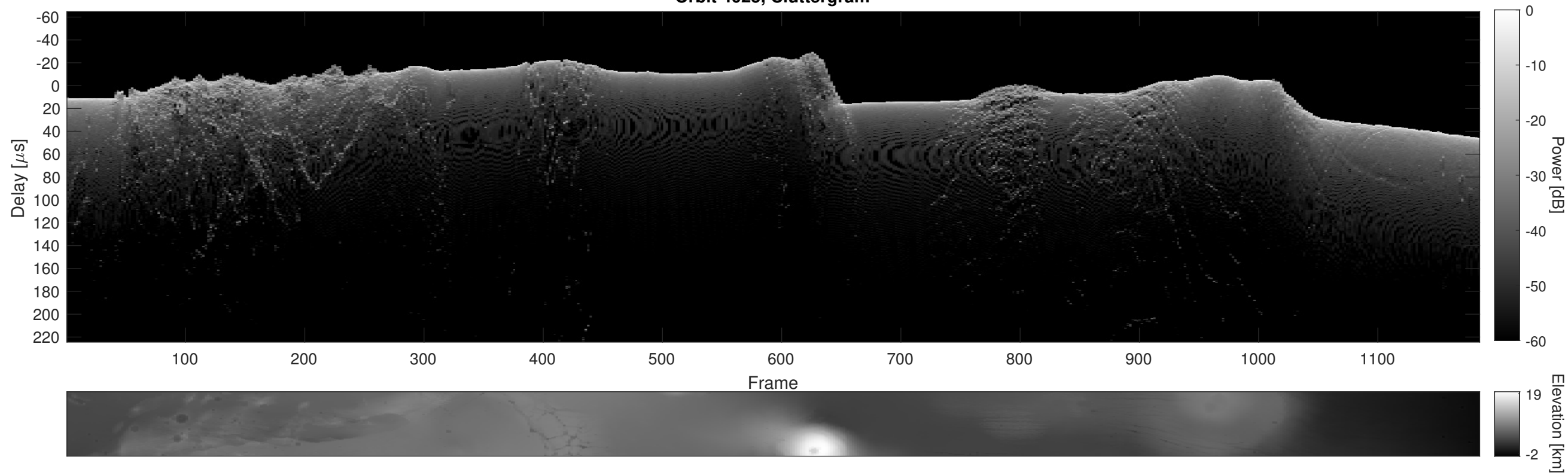
Orbit 4025, Cluttergram
