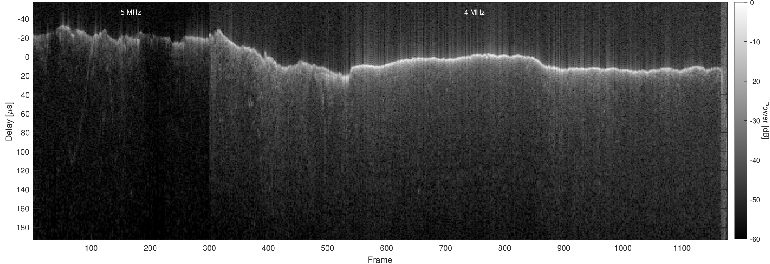
Orbit 4026, Chapman, No Window, Channel 2
