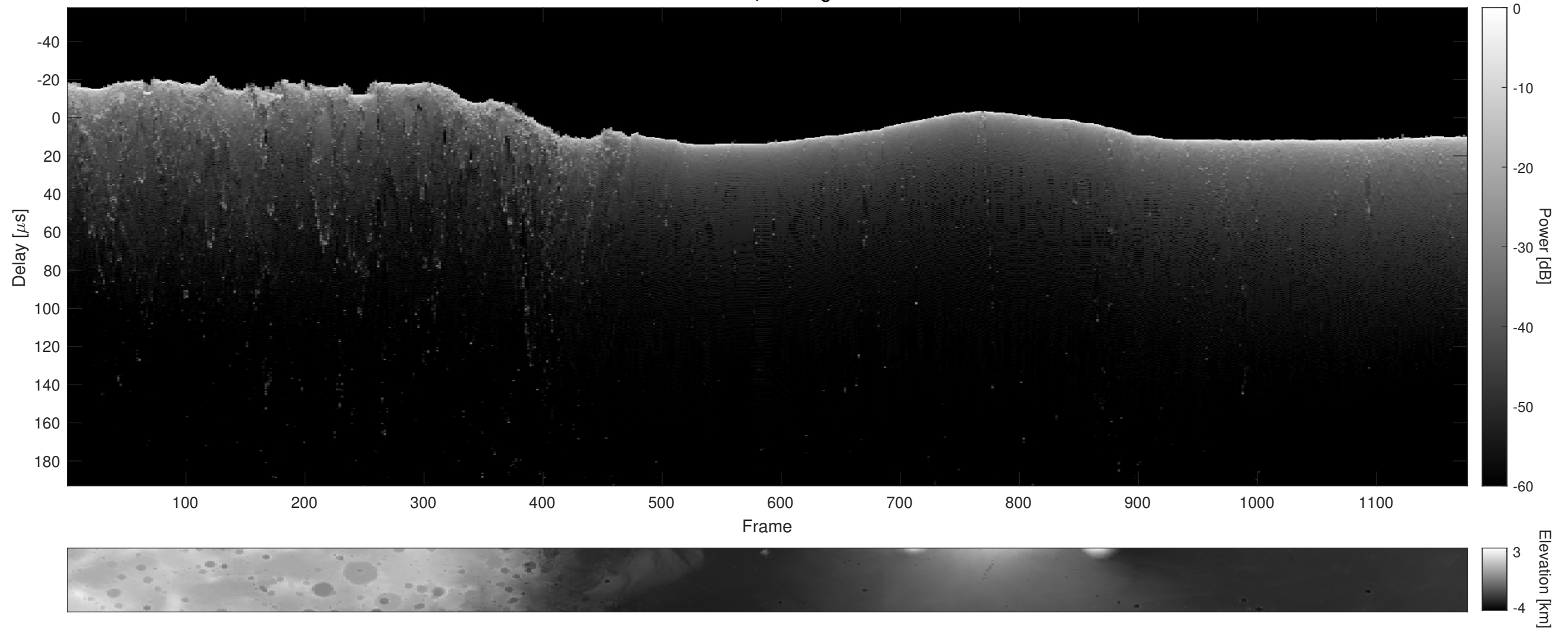
Orbit 4026, Cluttergram
