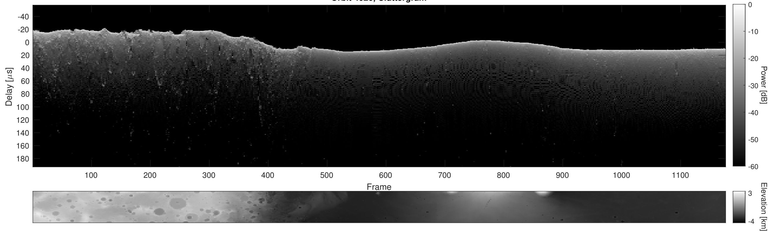
Orbit 4026, Cluttergram
