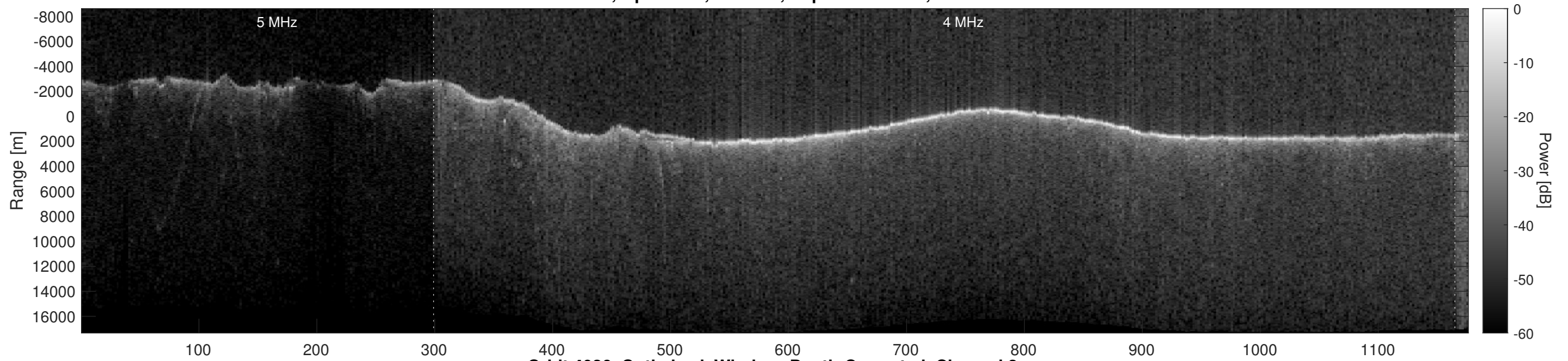
Orbit 4026, Optimized, Window, Depth-Corrected, Channel 2
