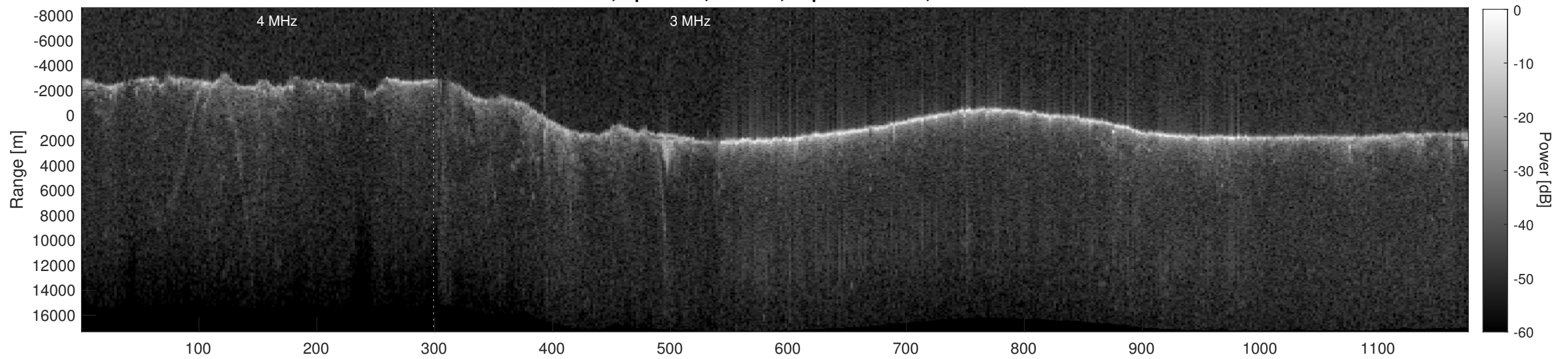
Orbit 4026, Depth-Corrected Cluttergram
