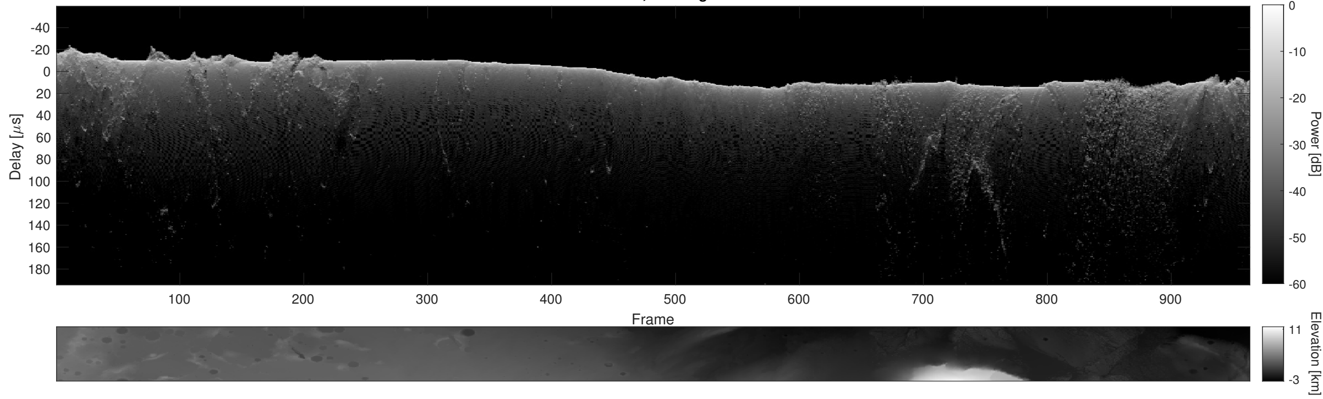
Orbit 4029, Cluttergram
