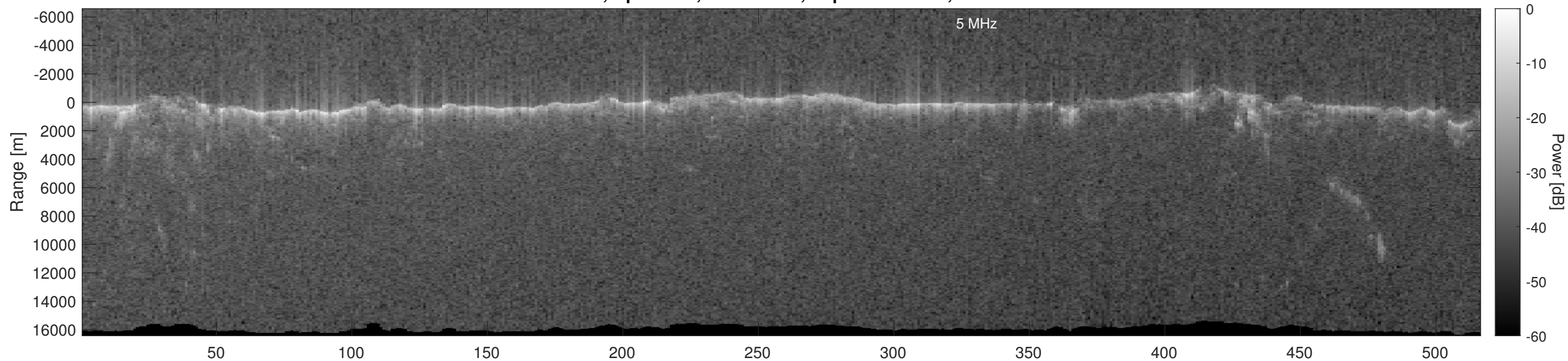
Orbit 4030, Optimized, No Window, Depth-Corrected, Channel 2
