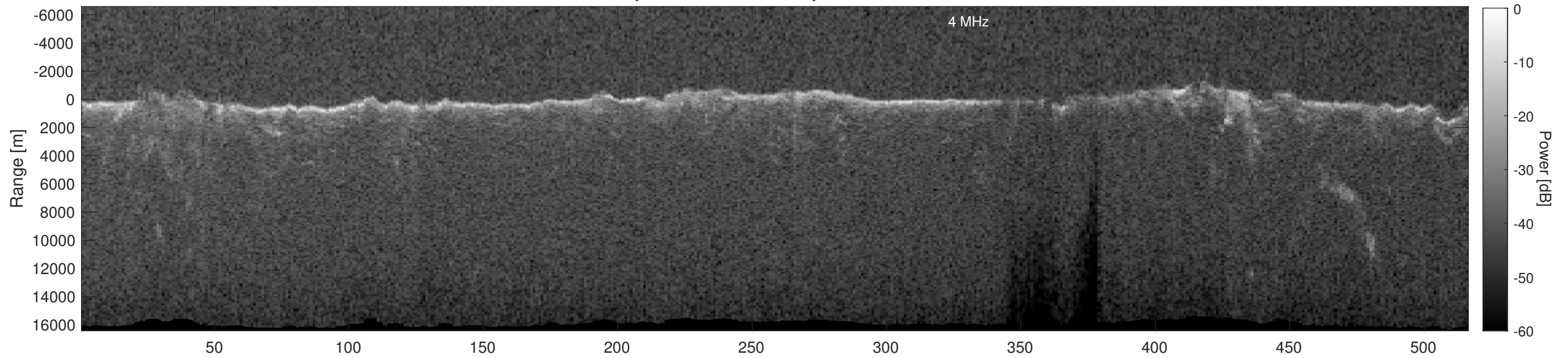
Orbit 4030, Depth-Corrected Cluttergram
