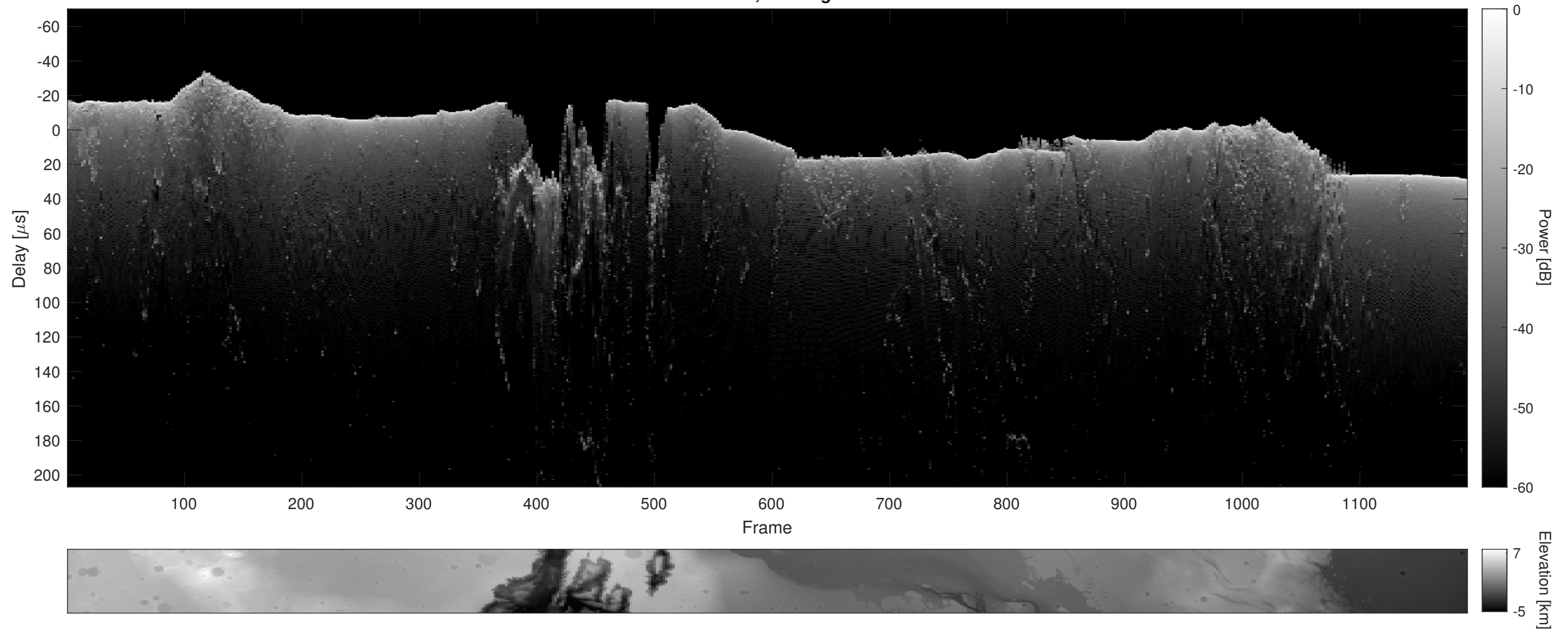
Orbit 4032, Cluttergram
