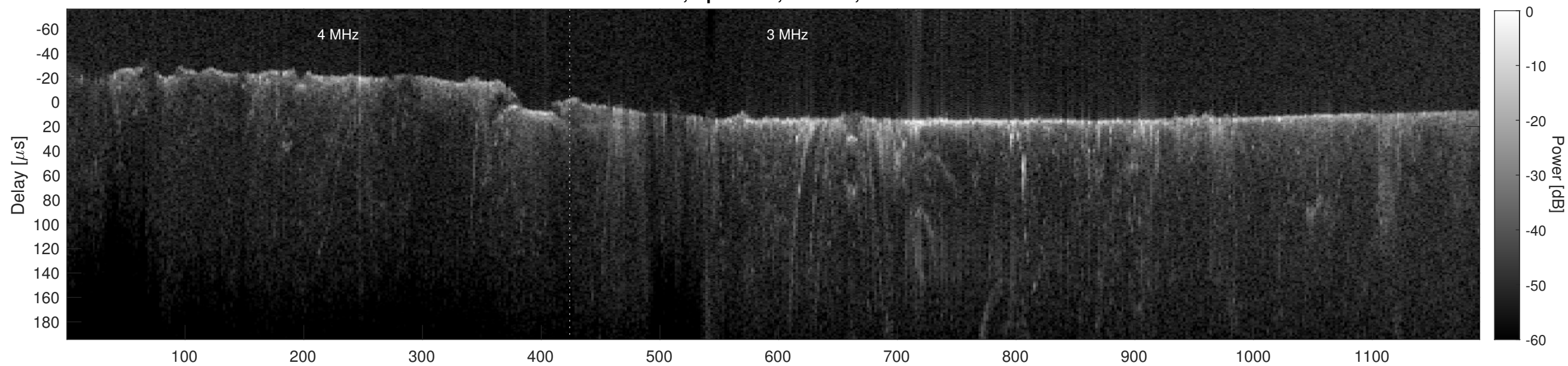
Orbit 4033, Cluttergram
