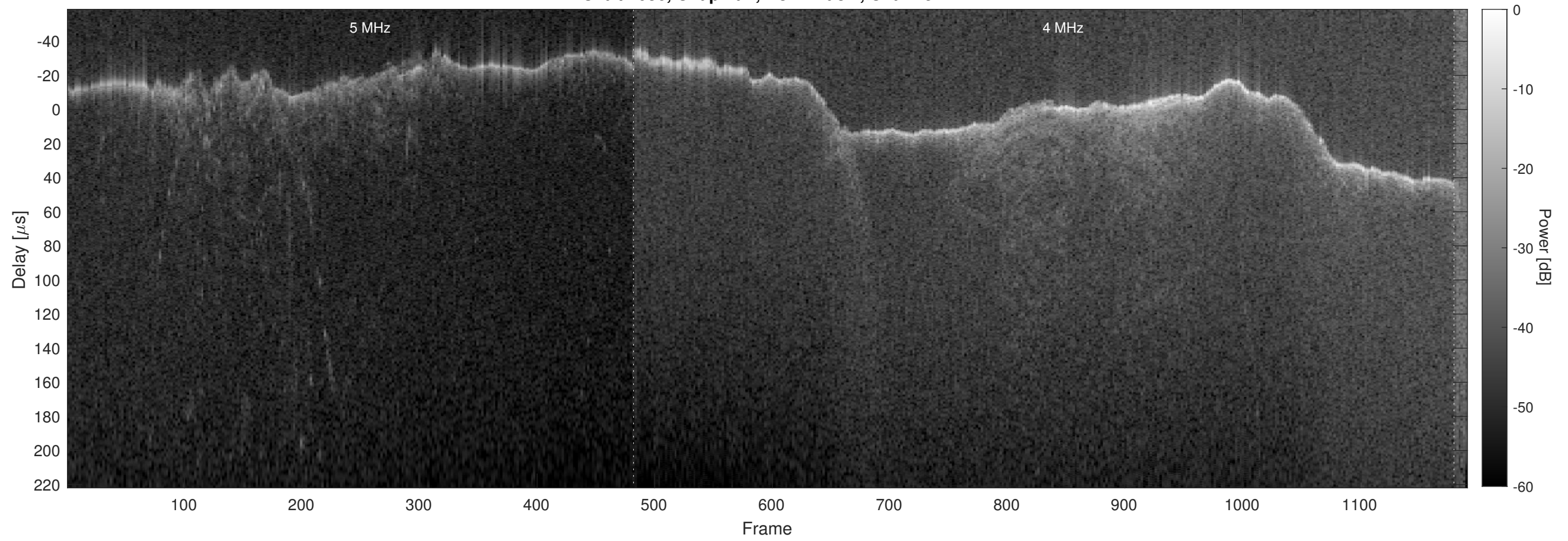
Orbit 4036, Chapman, No Window, Channel 2
