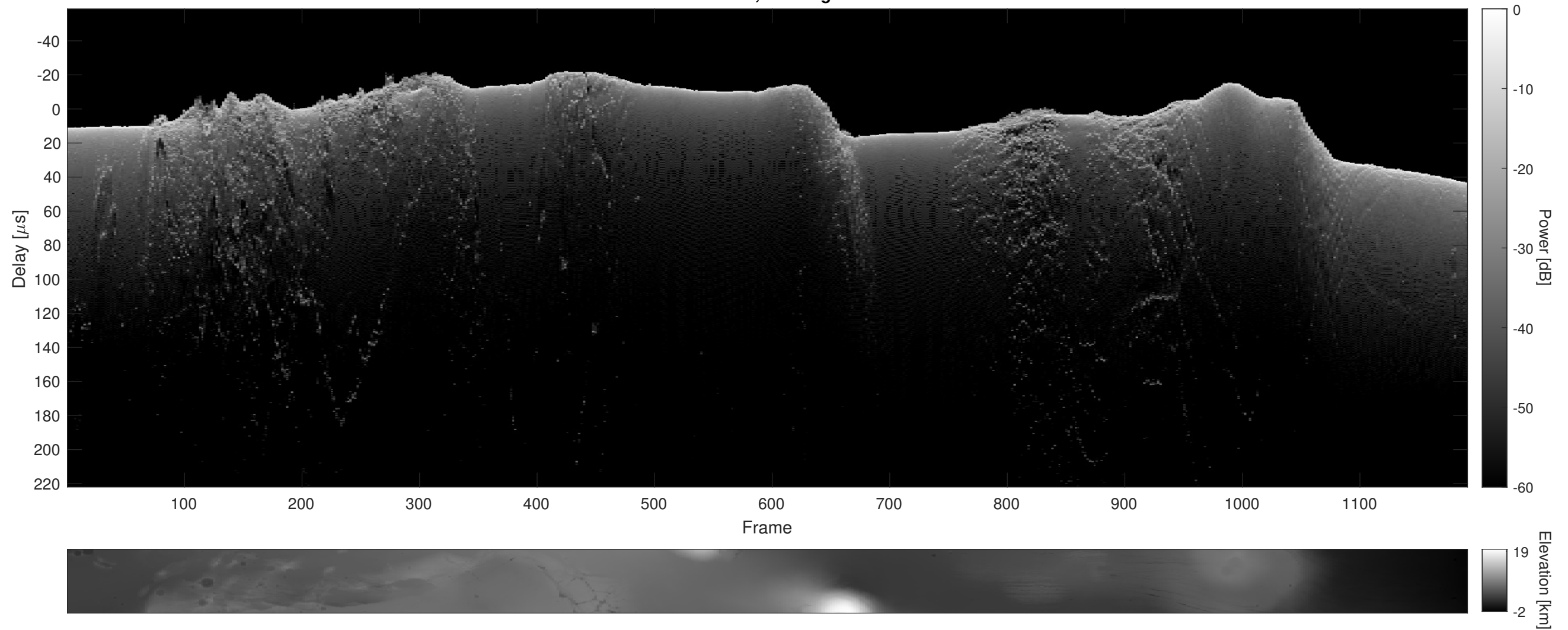
Orbit 4036, Cluttergram
