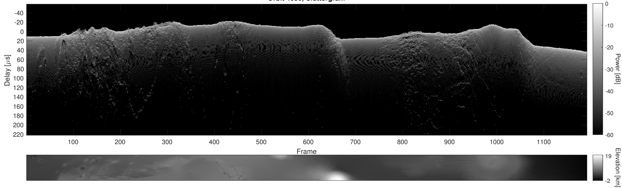
Orbit 4036, Cluttergram
