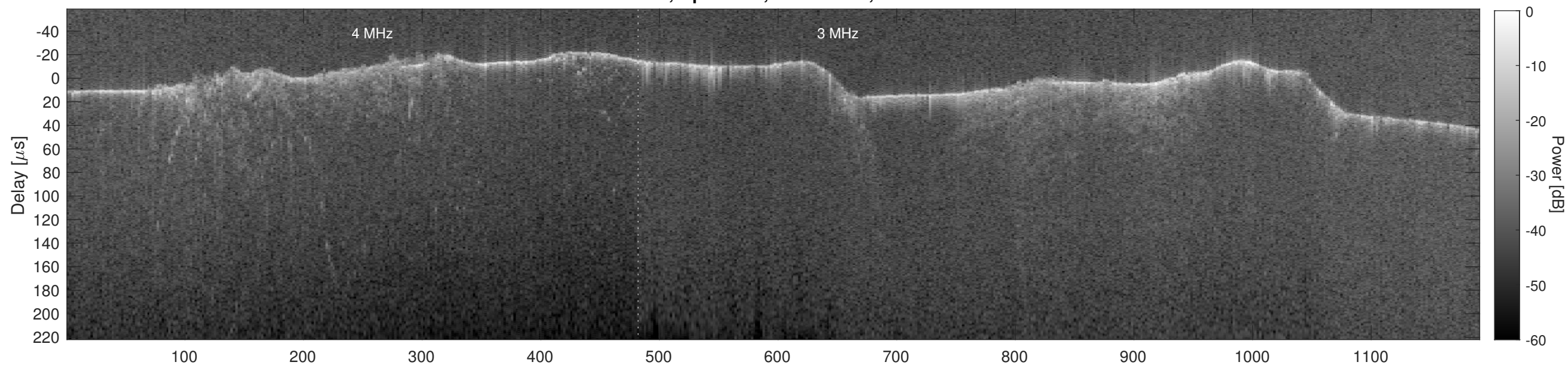
Orbit 4036, Cluttergram
