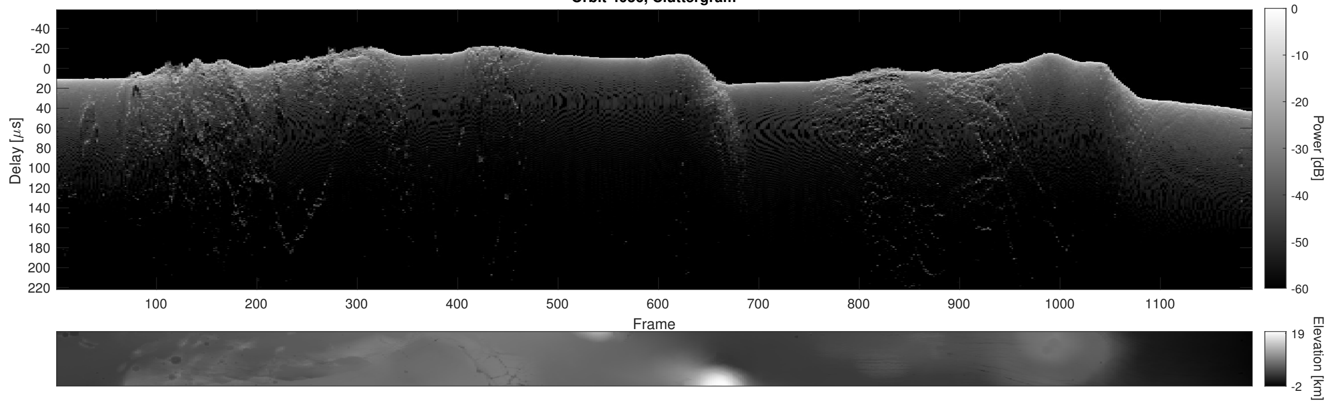
Orbit 4036, Cluttergram
