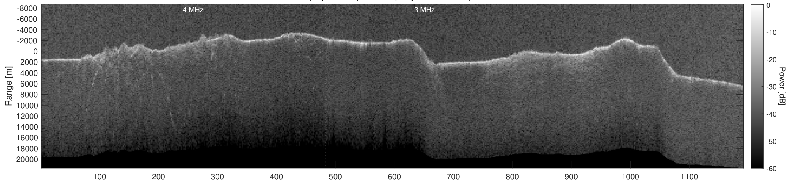
Orbit 4036, Depth-Corrected Cluttergram
