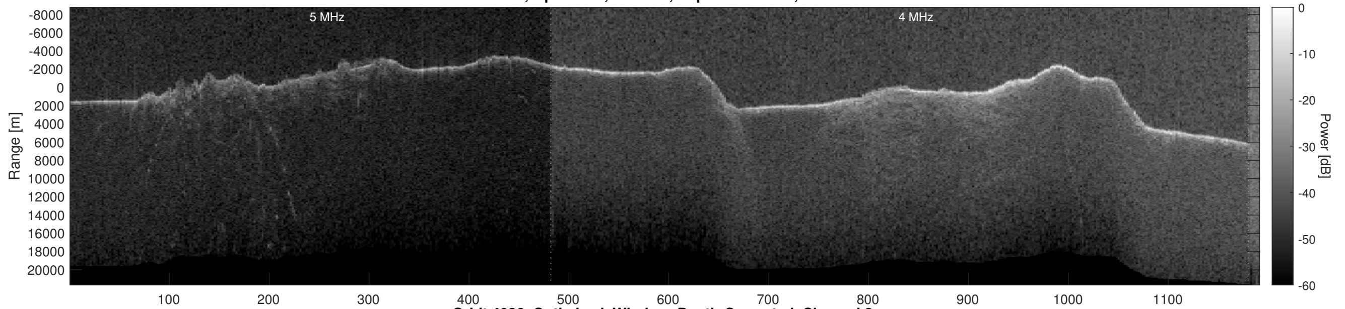
Orbit 4036, Optimized, Window, Depth-Corrected, Channel 2
