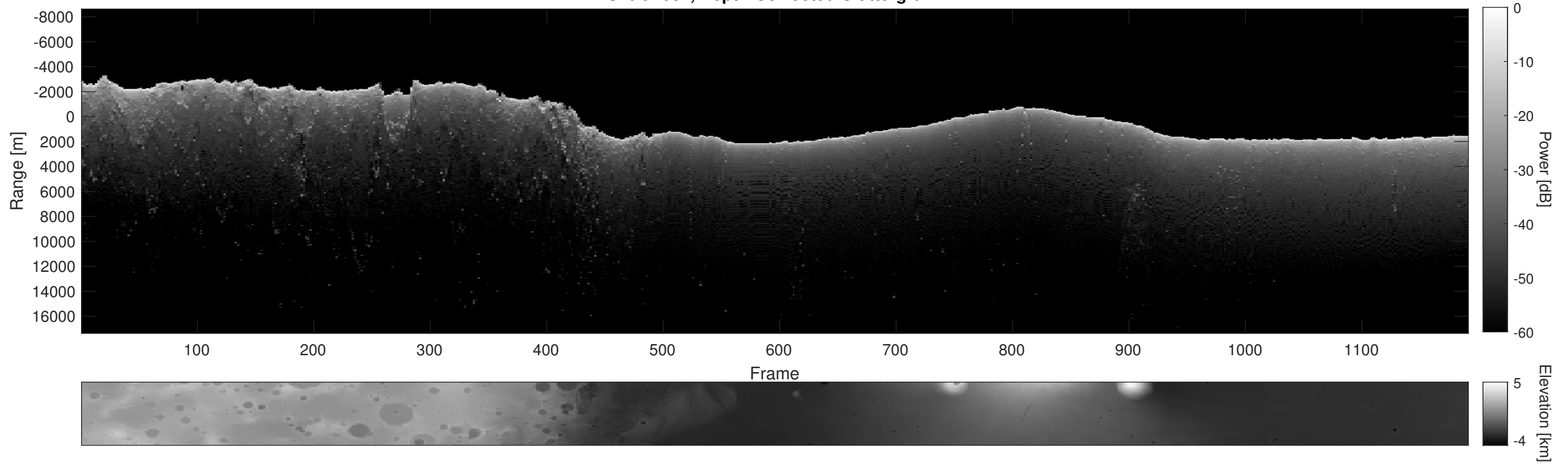
Orbit 4037, Depth-Corrected Cluttergram
