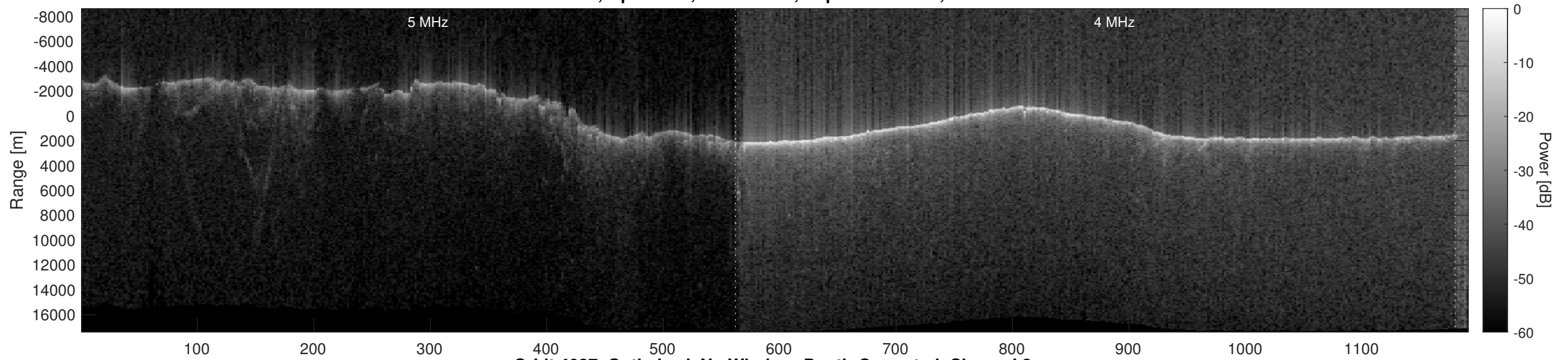
Orbit 4037, Optimized, No Window, Depth-Corrected, Channel 2
