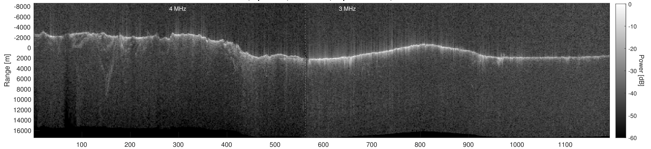
Orbit 4037, Depth-Corrected Cluttergram
