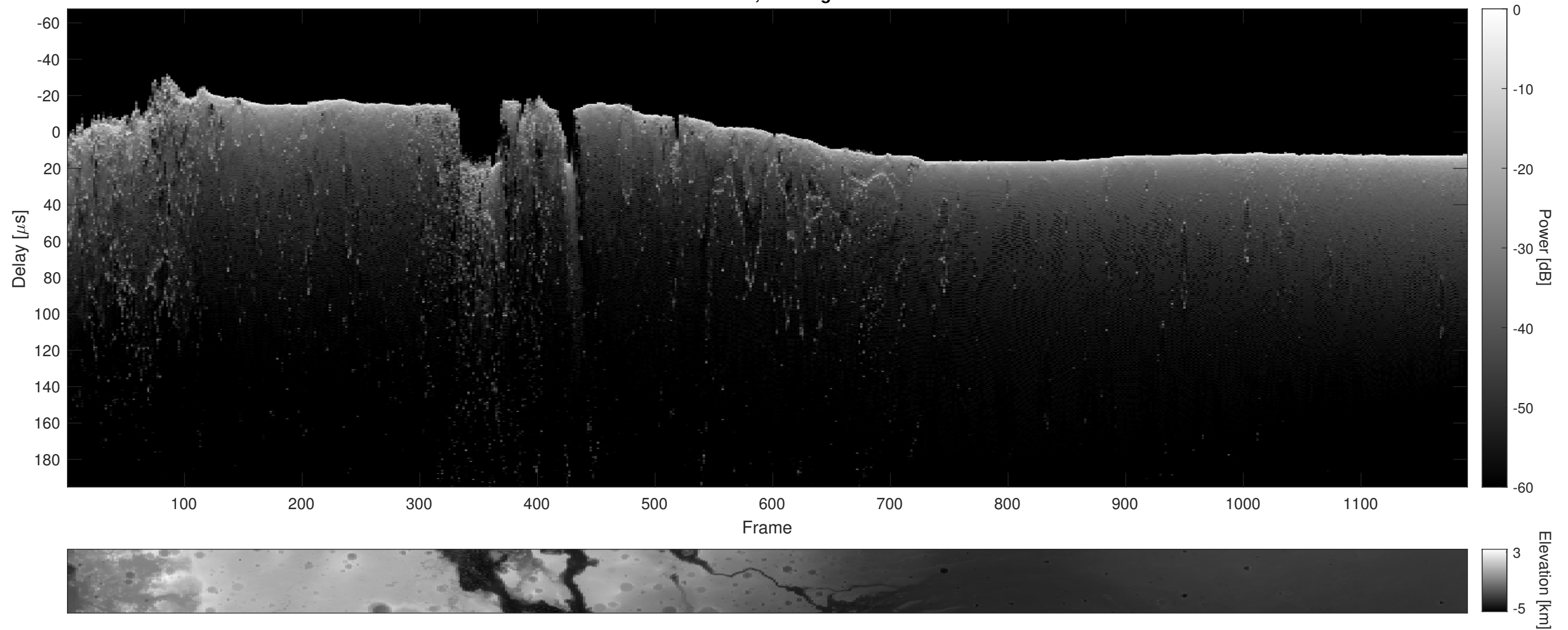
Orbit 4039, Cluttergram
