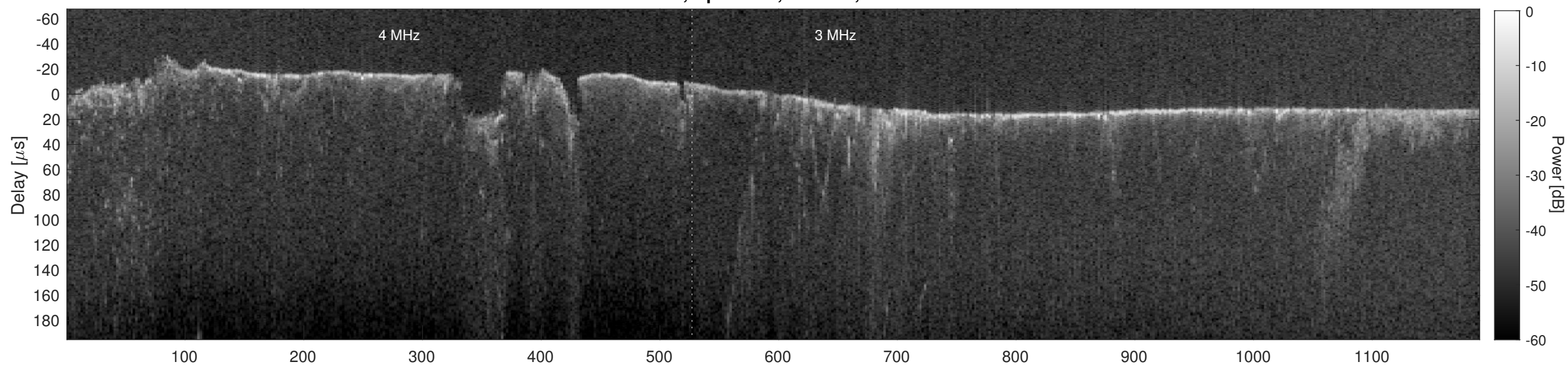
Orbit 4039, Cluttergram
