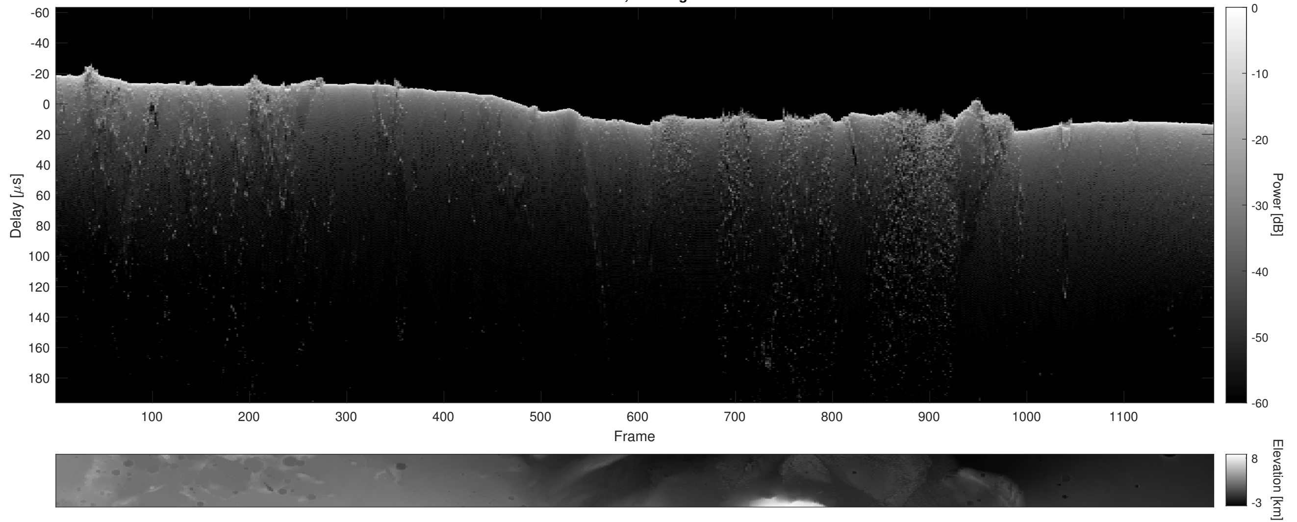
Orbit 4040, Cluttergram
