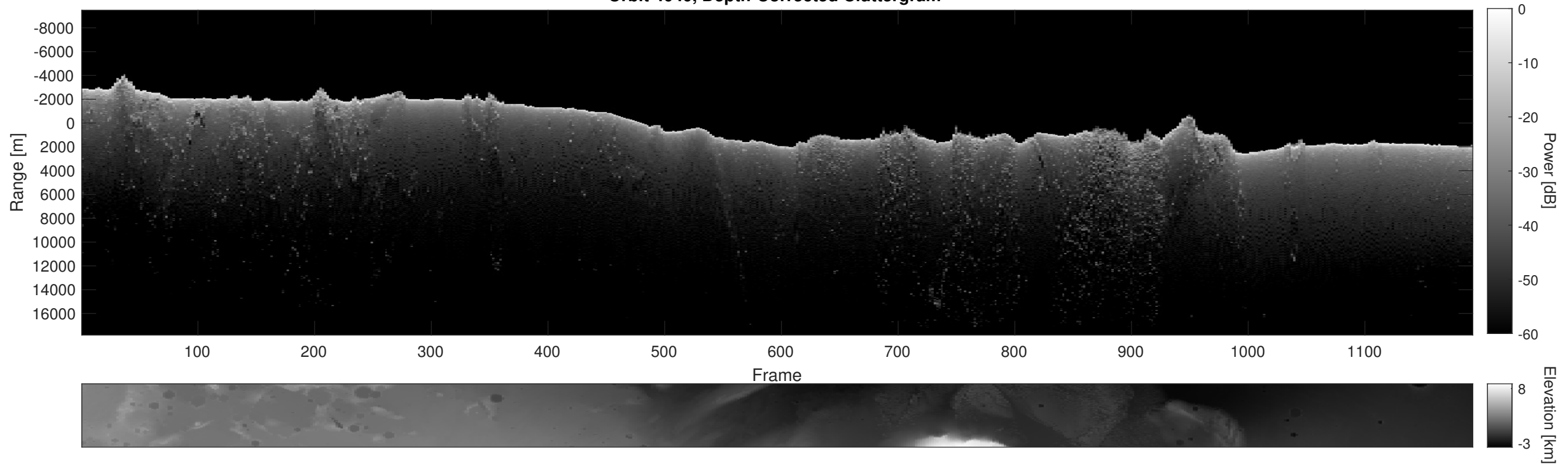
Orbit 4040, Depth-Corrected Cluttergram
