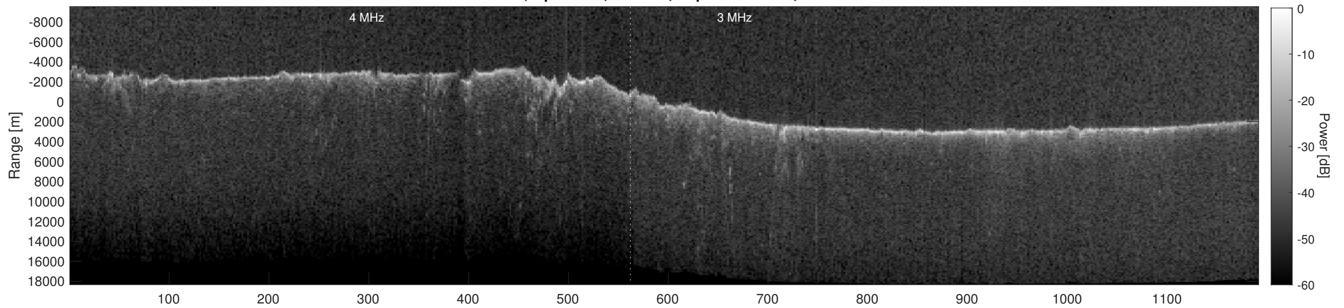
Orbit 4041, Depth-Corrected Cluttergram
