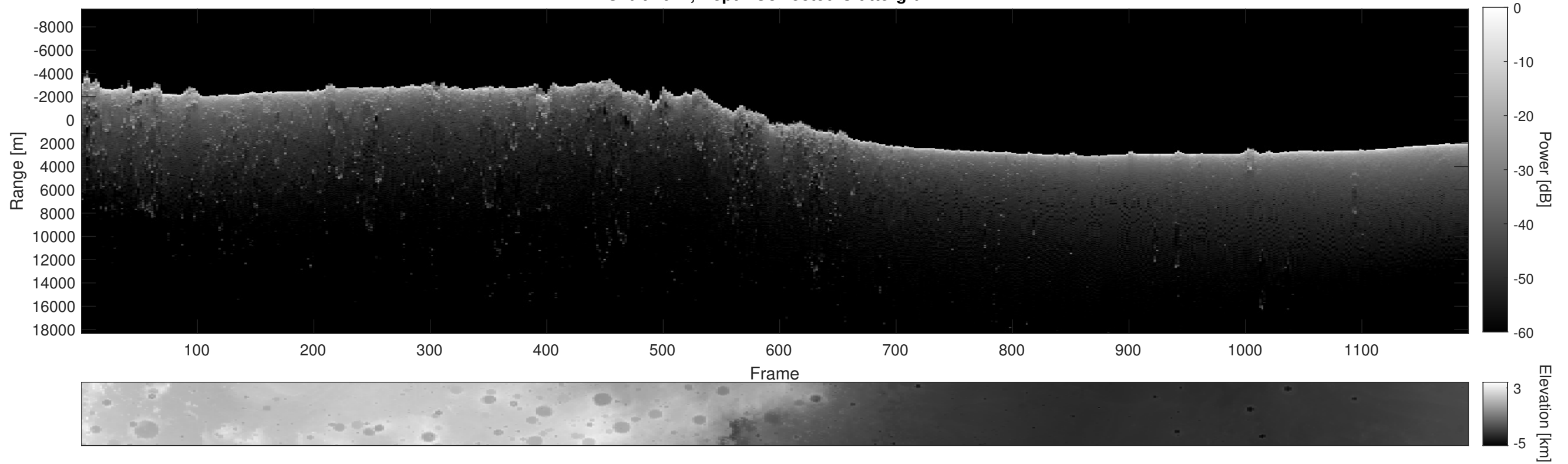
Orbit 4041, Depth-Corrected Cluttergram
