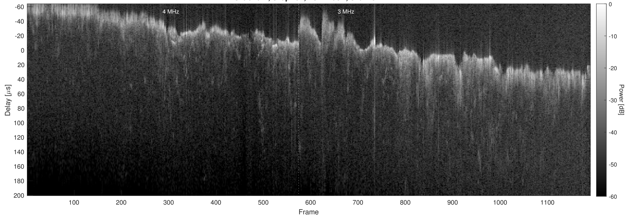
Orbit 4042, Chapman, No Window, Channel 2
