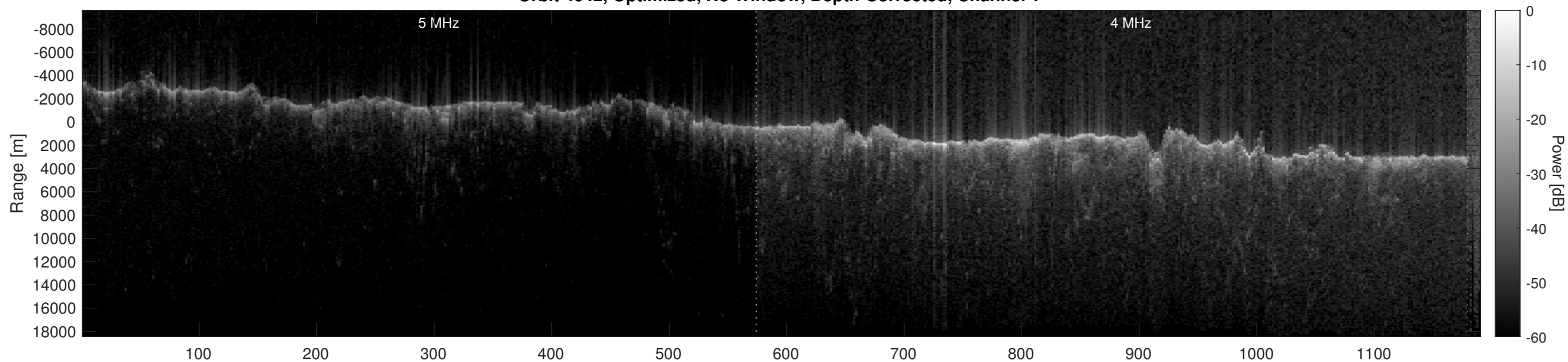
Orbit 4042, Optimized, No Window, Depth-Corrected, Channel 2
