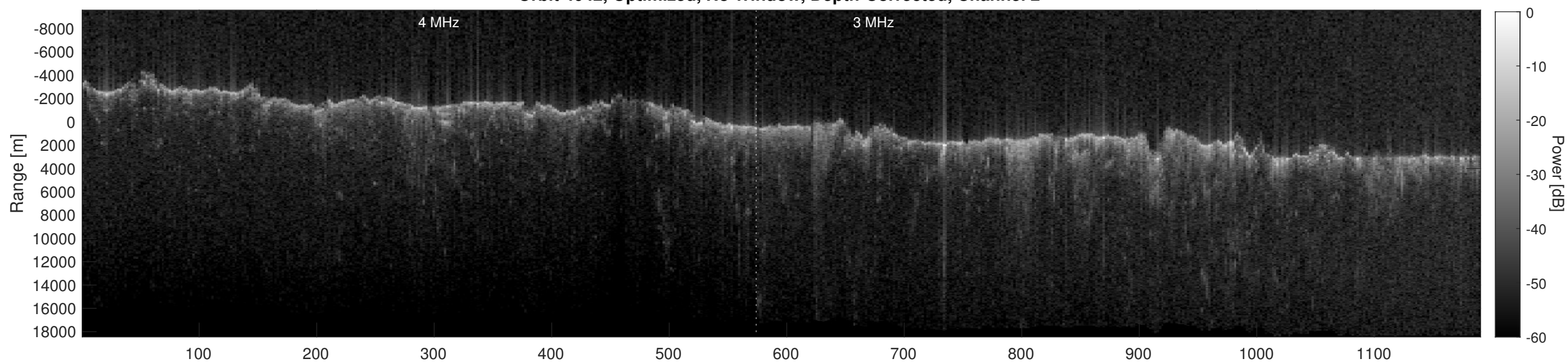
Orbit 4042, Depth-Corrected Cluttergram
