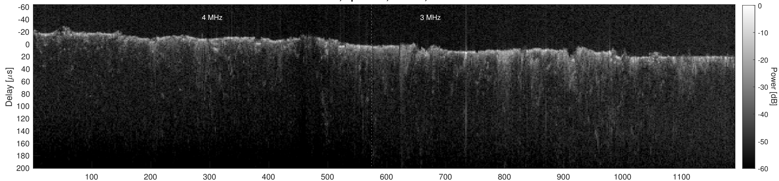
Orbit 4042, Cluttergram
